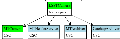
Main Telescope Architecture V3.0 Apr 10, 2019
